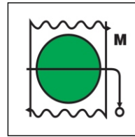
Fire damper M for machinery space
